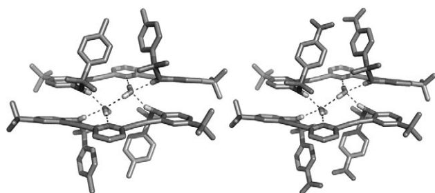
Figure 1. Crystal structures of receptors (1 \cdot H_2O)_2 (left) and (2 \cdot H_2O)_2 (right) illustrate the 2+2 dimer formed with water. The hydrogen bonds involving water as the donor atom form a helical twist through the center of the binding cavity. All hydrogen bonds are depicted as dashes. For clarity, H atoms not involved in hydrogen bonds were omitted, and only one position for the disordered H atom in the bridging solvent water molecule is shown.
