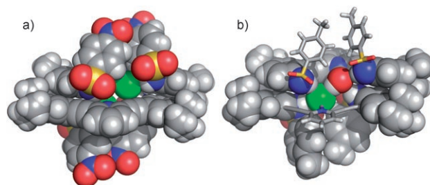
Figure 2. a) Space-filling representation of the crystal structure of (H2^+ \cdot Cl^-)_2 . b) Crystal structure of the water–chloride heterodimer (H1^+ \cdot Cl^-) \cdot (1 \cdot H_2O) . Both water and hydrogen chloride stabilize dimer formation, with seven hydrogen bonds within the binding cavity of the heterodimer. Only one position of the disordered water molecule and chloride ion is shown for clarity. Cl green, S yellow, N blue, O red, C gray, H light gray.
