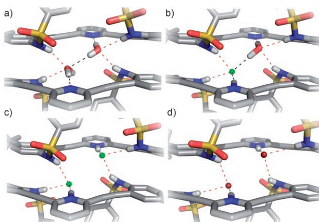
Figure 3. Wireframe representations of the crystal structures of a) (1 \cdot H_2O)_2 , b) (H1^+ \cdot Cl^-) \cdot (1 \cdot H_2O) , c) (H2^+ \cdot Cl^-)_2 , and d) (H1^+ \cdot Br^-)_2 highlighting the interchangeable role that halides and water play in the dimerization of 2,6-bis(2-anilinoethynyl)pyridine sulfonamide receptors. Hydrogen bonds are illustrated as dashes (sulfonamide in red and all others in black). Hydrogen atoms not involved in H-bonds are omitted for clarity. Cl green, Br maroon, S yellow, N blue, O red, C gray, H light gray.
